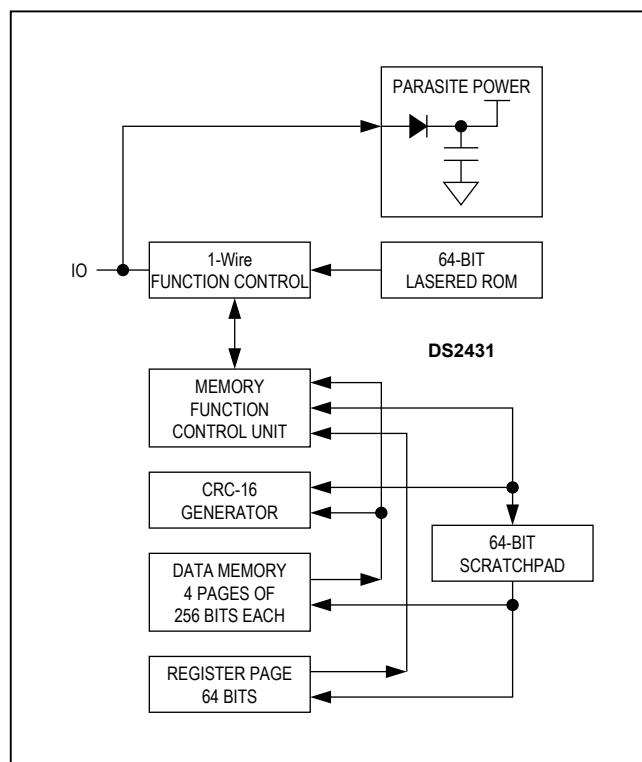
Figure 1. Block Diagram
