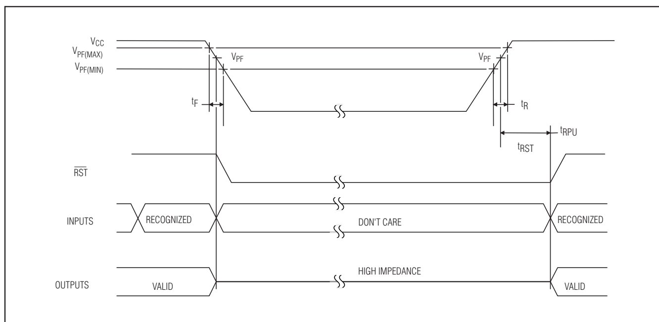
Figure 1. Power-Up/Down Timing
