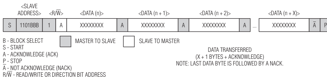
Figure 8. Data Read—Slave Transmitter Mode
