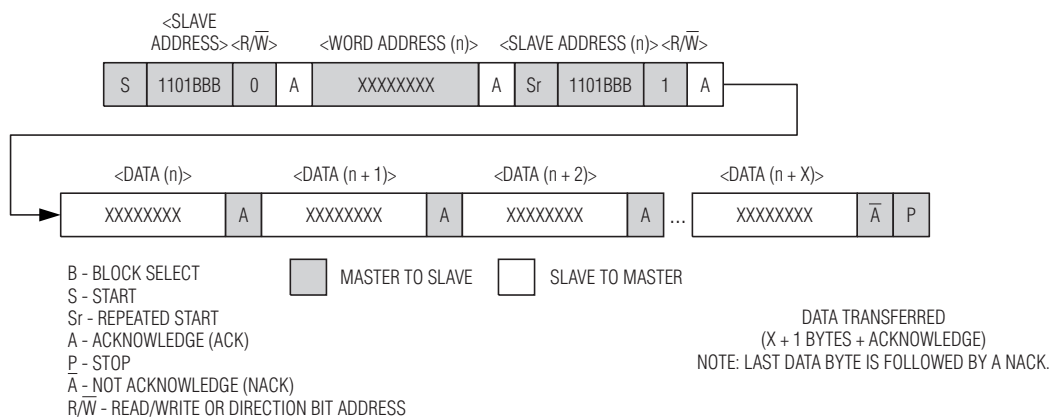
Figure 9. Data Write/Read (Write Pointer, Then Read)—Slave Receive and Transmit
