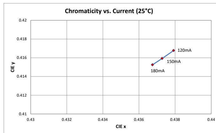
Chromaticity vs Current
