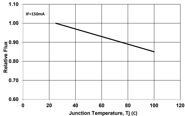
Tj-----Relative Luminous Flux
