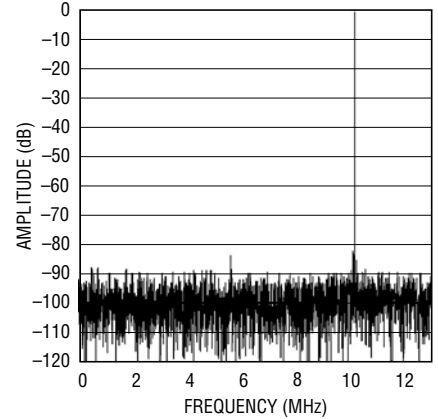
LTC2286: 8192 Point FFT, f_{IN} = 140\text{MHz} , -1\text{dB} , 2V Range, 25Msps
