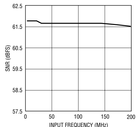
LTC2287: SNR vs Input Frequency, -1dB, 2V Range, 40Msps
