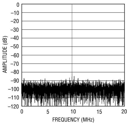
LTC2287: 8192 Point FFT, f_{IN} = 30\text{MHz} , -1dB, 2V Range, 40Msps
