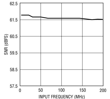
LTC2286: SNR vs Input Frequency, -1\text{dB} , 2V Range, 25Msps
