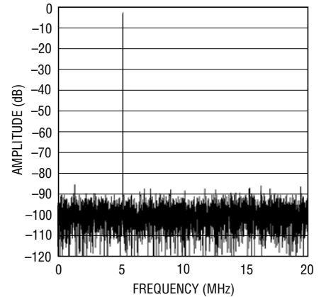
LTC2287: 8192 Point FFT, f_{IN} = 5\text{MHz} , -1dB, 2V Range, 40Msps
