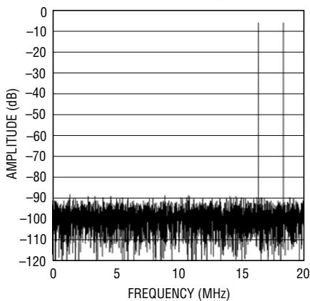
LTC2287: 8192 Point 2-Tone FFT, f_{IN} = 21.6\text{MHz} and 23.6\text{MHz} , -1dB, 2V Range, 40Msps
