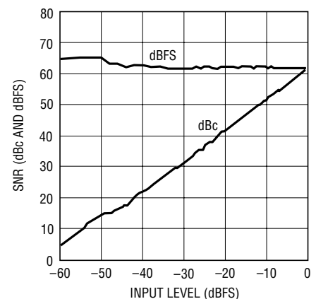
LTC2286: SNR vs Input Level, f_{IN} = 5\text{MHz} , 2V Range, 25Msps
