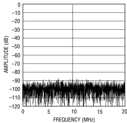
LTC2287: 8192 Point FFT, f_{IN} = 70\text{MHz} , -1dB, 2V Range, 40Msps
