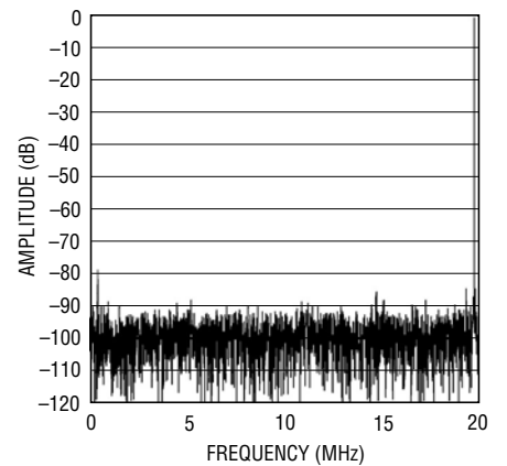
LTC2287: 8192 Point FFT, f_{IN} = 140\text{MHz} , -1dB, 2V Range, 40Msps
