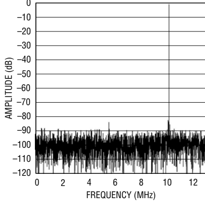
LTC2286: 8192 Point FFT, f_{IN} = 70\text{MHz} , -1\text{dB} , 2V Range, 25Msps
