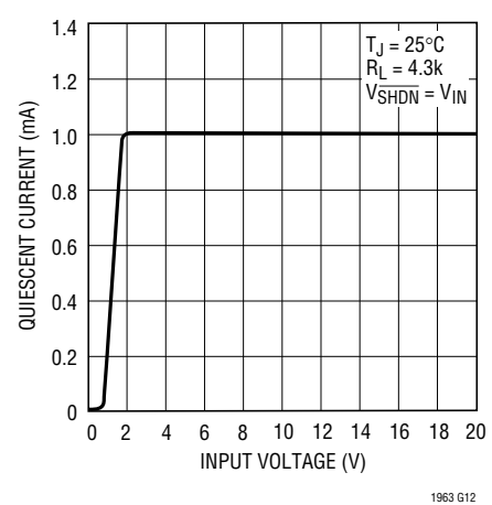
LT1963 Quiescent Current
