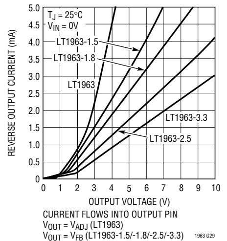
Reverse Output Current
