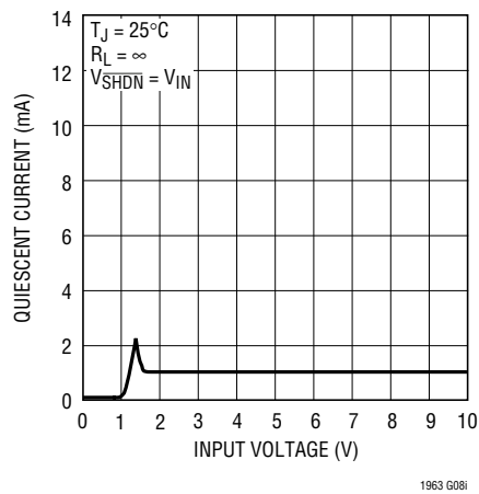
LT1963-3.3 Quiescent Current
