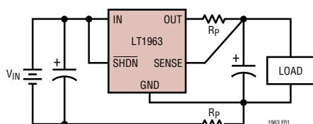
Figure 1. Kelvin Sense Connection
