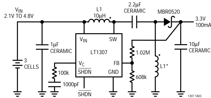
Step-Up/Step-Down Converter
