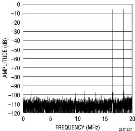
LTC2247: 8192 Point 2-Tone FFT, f_{IN} = 21.6\text{MHz} and 23.6\text{MHz} , -1\text{dB} , 2V Range, 40Msps
