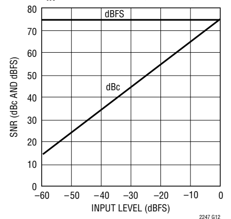
LTC2247: SNR vs Input Level, f_{IN} = 5\text{MHz} , 2V Range, 40Msps
