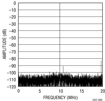
LTC2247: 8192 Point FFT, f_{IN} = 70\text{MHz} , -1\text{dB} , 2V Range, 40Msps
