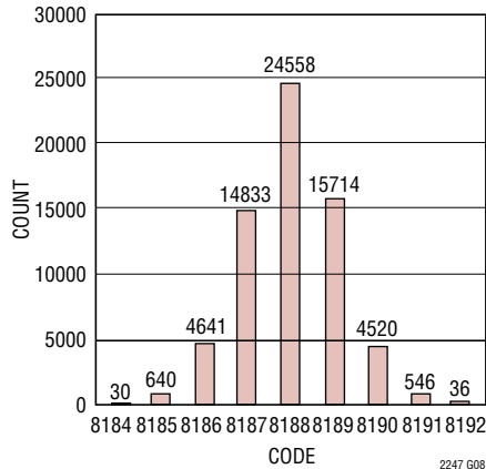
LTC2247: Grounded Input Histogram, 40Msps
