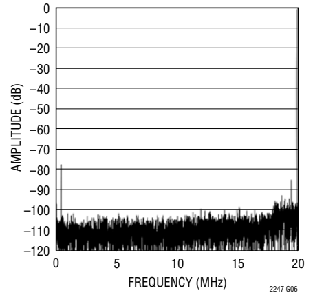
LTC2247: 8192 Point FFT, f_{IN} = 140\text{MHz} , -1\text{dB} , 2V Range, 40Msps
