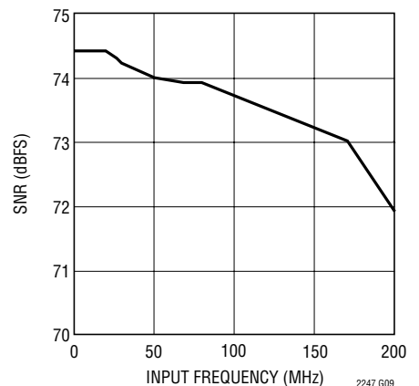
LTC2247: SNR vs Input Frequency, -1\text{dB} , 2V Range, 40Msps
