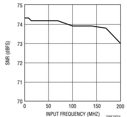
LTC2248: SNR vs Input Frequency, -1dB, 2V Range, 65Msps
