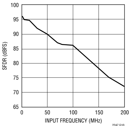
LTC2247: SFDR vs Input Frequency, -1\text{dB} , 2V Range, 40Msps
