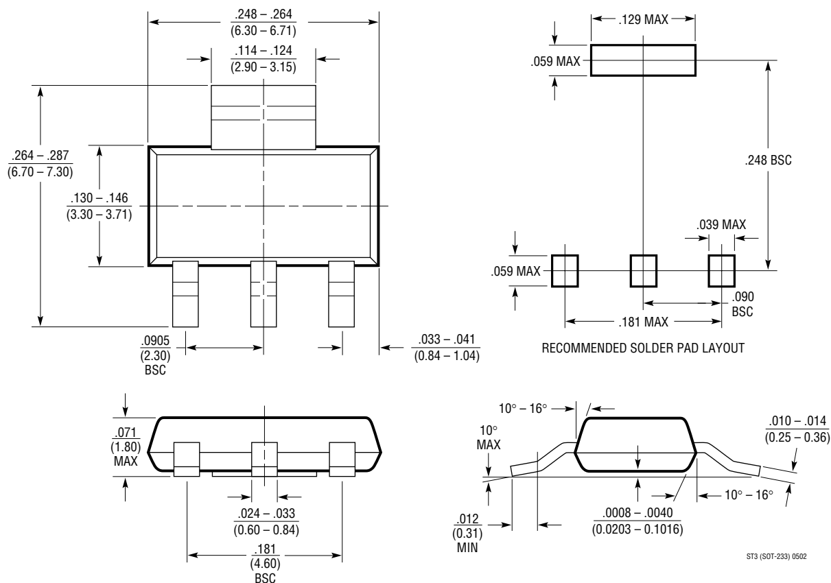
ST Package 3-Lead Plastic SOT-223 (LTC DWG # 05-08-1630)
