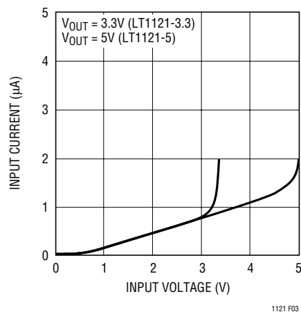
Figure 3. Input Current
