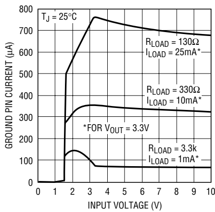
LT1121-3.3 Ground Pin Current
