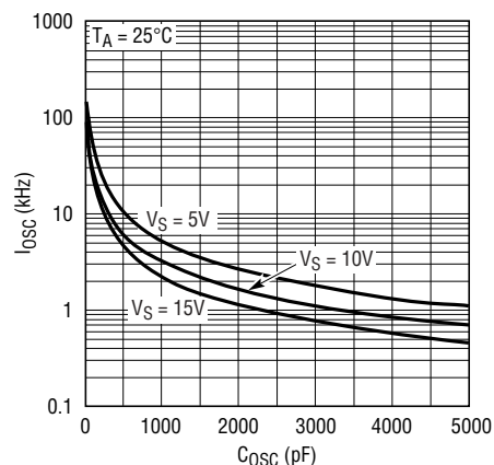
Oscillator Frequency, f_{osc} vs C_{osc}
