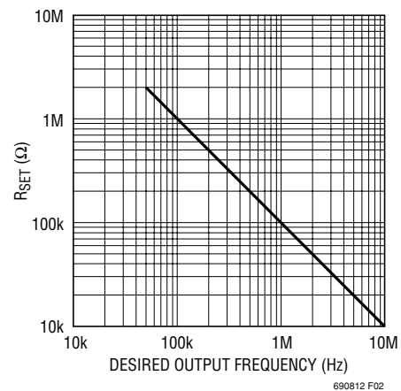
Figure 2. R_{\text{SET}} vs Desired Output Frequency
