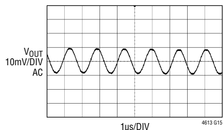
Output Ripple
