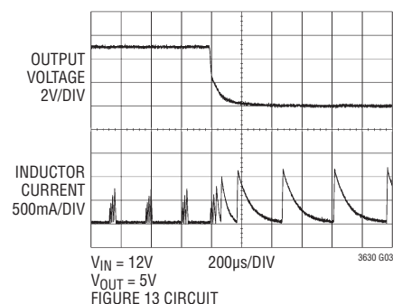
Short-Circuit Response
