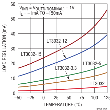
Negative Load Regulation
