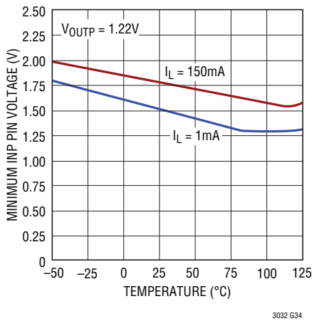
LT3032 Minimum INP Pin Voltage
