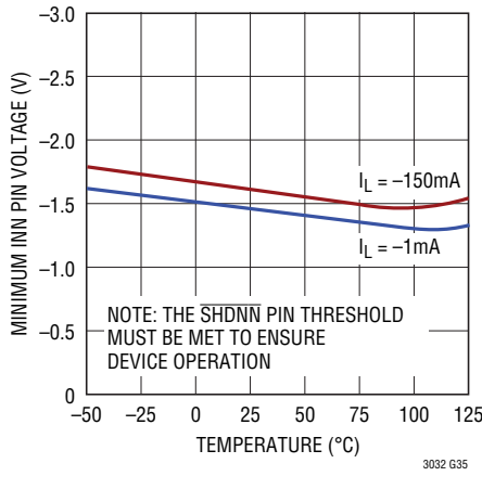
LT3032 Minimum INN Pin Voltage
