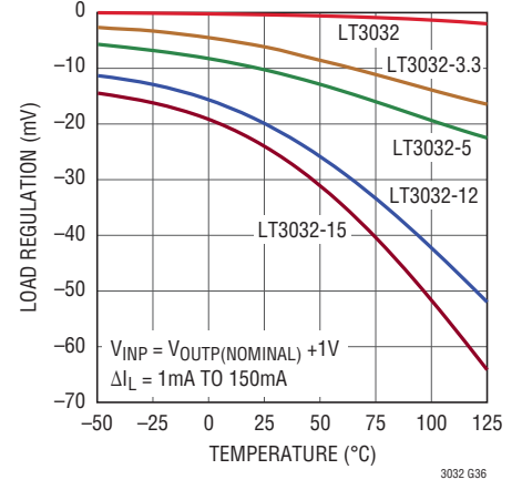
Positive Load Regulation
