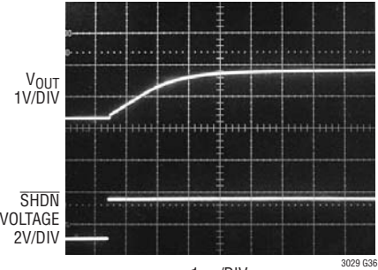
Start-Up Time from Shutdown, C_{BYP} = 0.01\mu\text{F}
