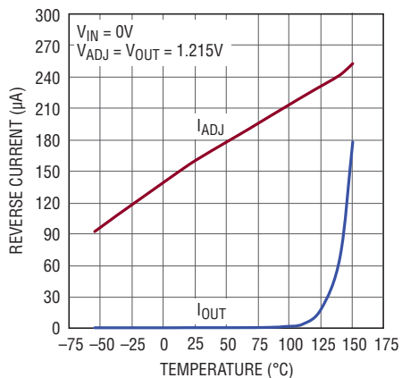
Reverse Current
