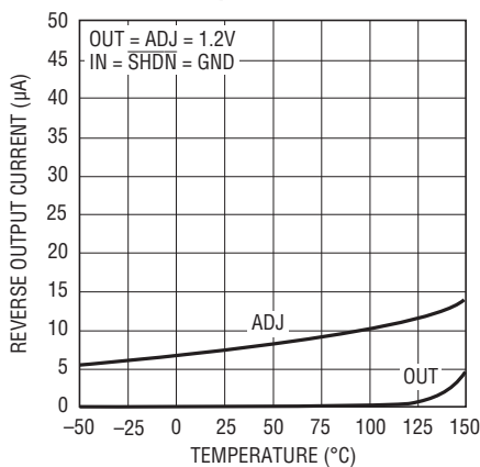
Reverse-Output Current
