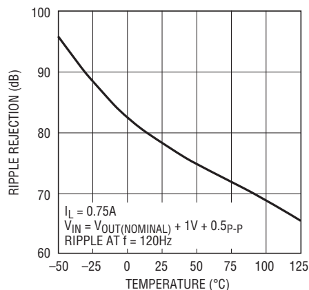
Ripple Rejection vs Temperature
