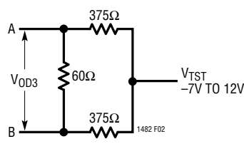
Figure 2. Driver DC Test Load #2
