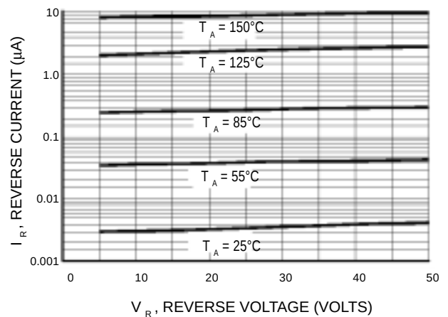
Figure 3. Leakage Current
