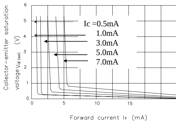
Fig. 3 Collector-emitter Saturation Voltage vs. Forward Current ( T_a=25^\circ\text{C} )
