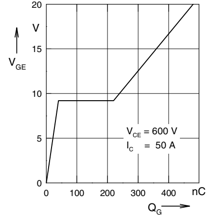
Fig. 9 Typ. turn on gate charge
