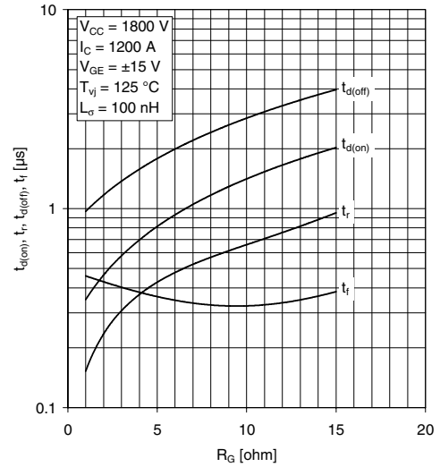
Fig. 10 Typical switching times vs gate resistor
