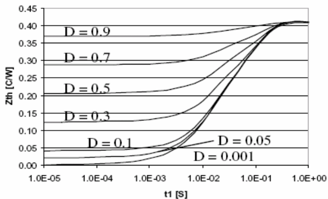
IXZ210N50L Thermal Response
