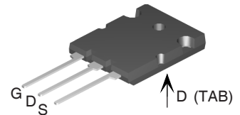
TO-264(SP) (IXTK)
