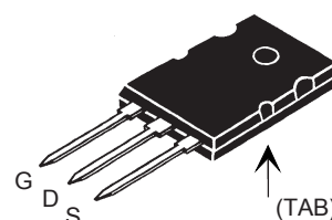
TO-264 (IXTK)
