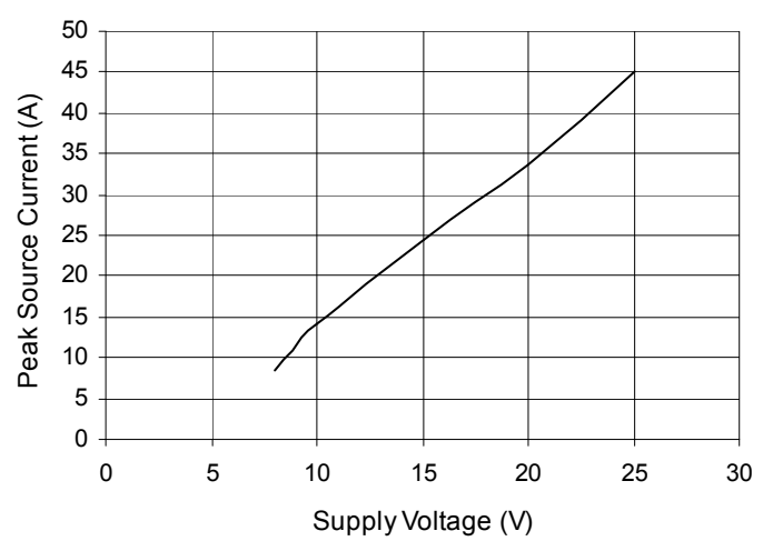
Fig. 15 Peak Source Current vs. Supply Voltage
