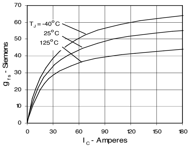
Fig. 7. Transconductance
