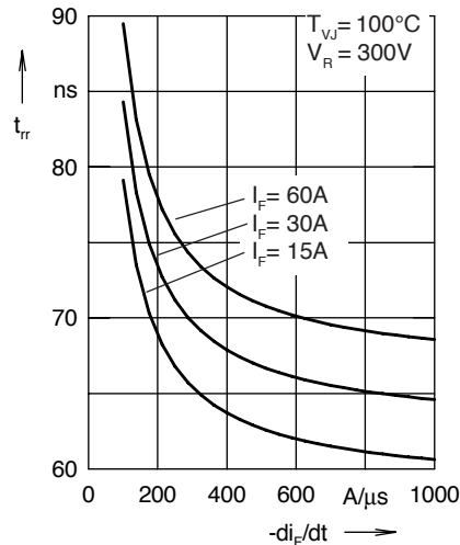
Fig. 18. Recovery time t_{rr} versus -di_F/dt
