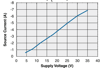
Output Source Current vs. Supply Voltage ( C_L=27nF )
