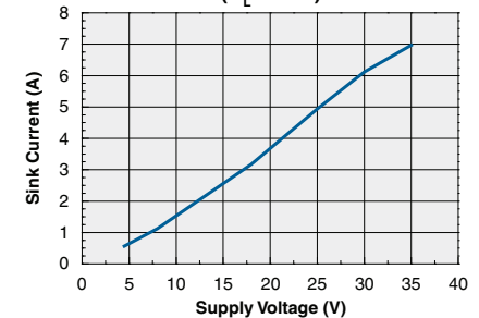
Output Sink Current vs. Supply Voltage ( C_L=27nF )
