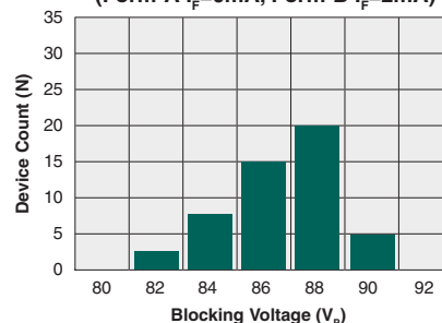
Typical Blocking Voltage Distribution (N=50, T_A=25^\circ\text{C} ) (Form-A I_F=0\text{mA} , Form-B I_F=2\text{mA} )
