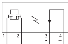
CPC1909J Pinout
