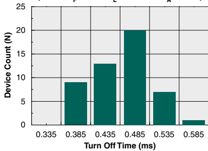
Typical Turn-On Time Distribution (N=50, I_F=5\text{mA} , I_L=100\text{mA} , T_A=25^\circ\text{C} )
