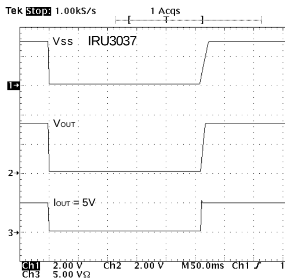
Figure 23 - Shutdown the output by pulling down the soft-start.
