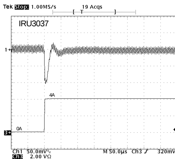
Figure 26 - Transient response @ I_{OUT} = 0 to 4A.
