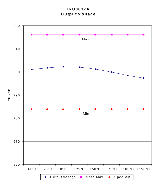
Figure 14 - Output Voltage
