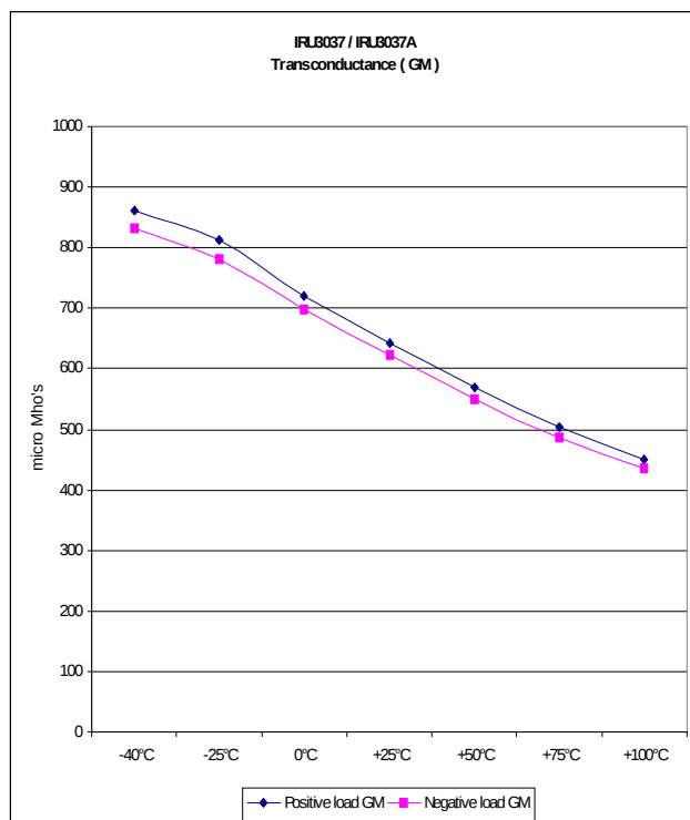
Figure 16 - Transconductance
