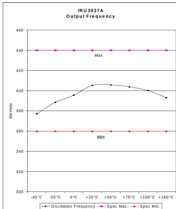
Figure 15 - Output Frequency
