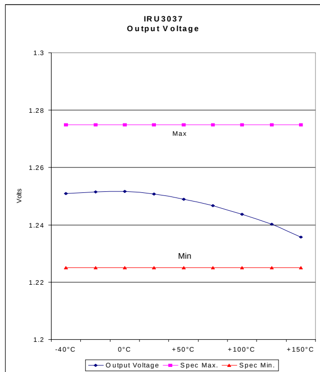
Figure 11 - Output Voltage
