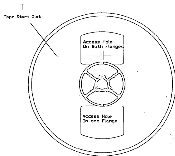
BACK VIEW
