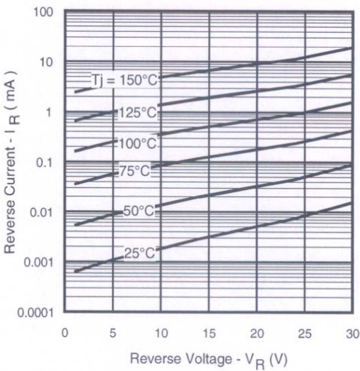
Fig. 12 - Typical Values of Reverse Current Vs. Reverse Voltage
