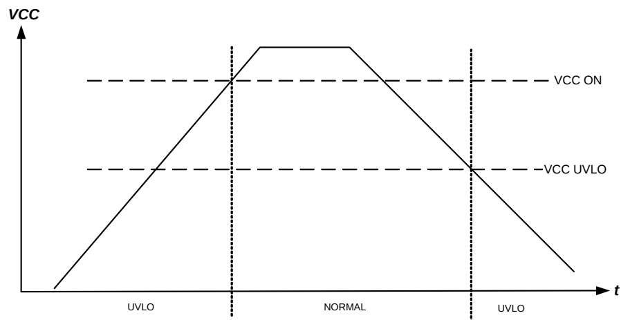
Figure 11: Vcc UVLO
