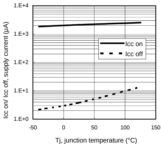
Figure 12 – I_{cc\ on}/I_{cc\ off} ( \mu\text{A} ) Vs T_j ( ^{\circ}\text{C} )
