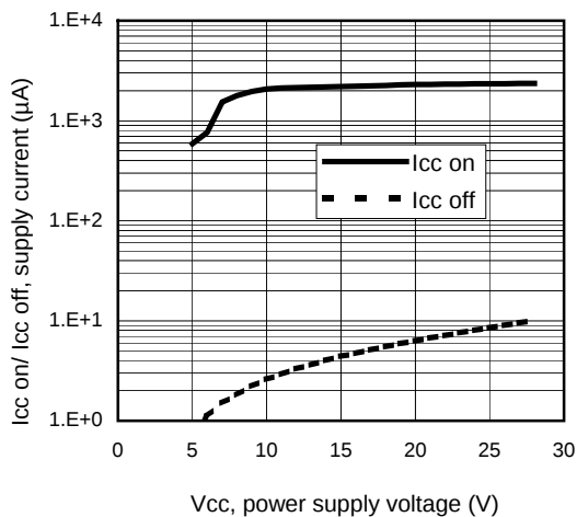
Figure 11 – I_{cc\ on}/I_{cc\ off} ( \mu\text{A} ) Vs V_{cc} (V)
