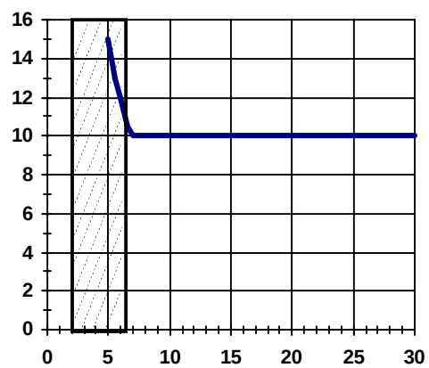
Figure 9- R_{dsON} ( \text{m}\Omega ) vs V_{cc-Vin} (V)
