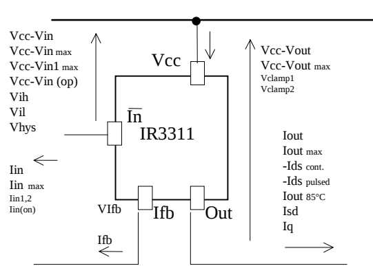
Figure 1 - Voltages and currents definitions
