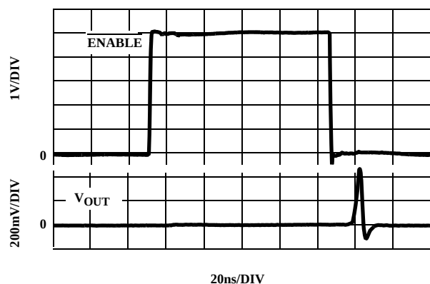
FIGURE 16. \overline{ENABLE} SWITCHING GLITCH V_{IN} = 0V , A_V = 2
