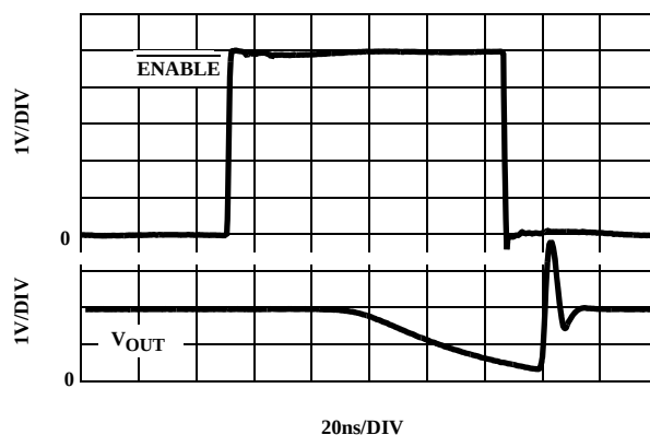
FIGURE 17. \overline{ENABLE} TRANSIENT RESPONSE V_{IN} = 1V , A_V = 2
