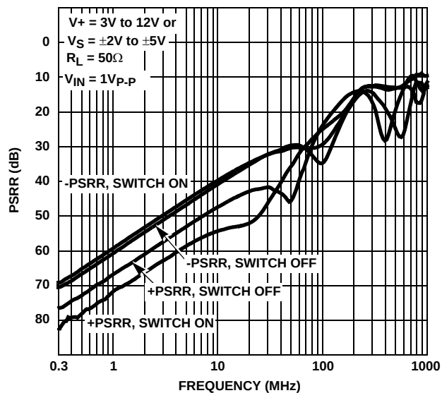
FIGURE 20. \pm PSRR vs FREQUENCY
