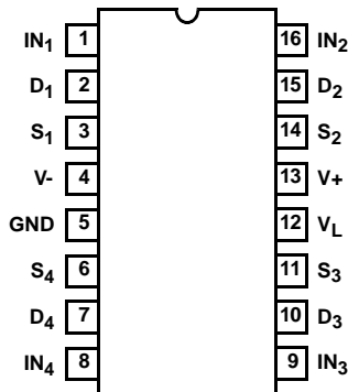
DG444, DG445 (SOIC) TOP VIEW
