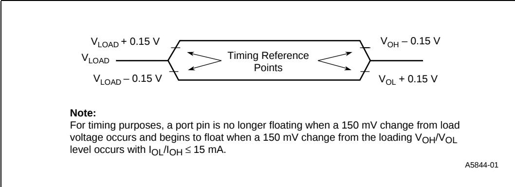
Figure 13. Float Waveforms
