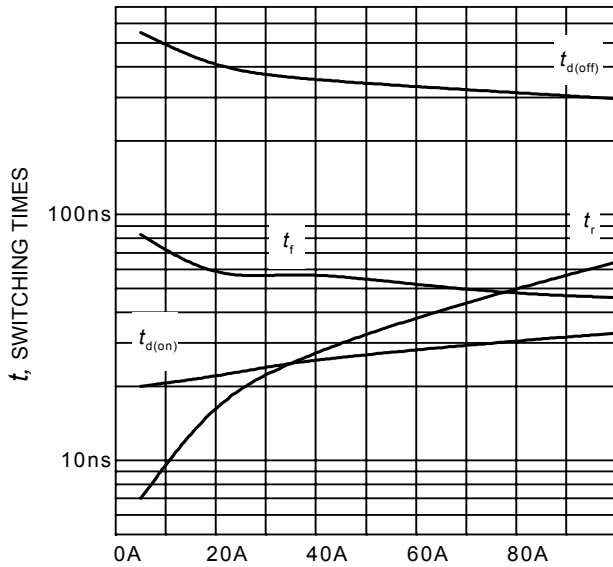
Figure 9. Typical switching times as a function of collector current (inductive load, T_J = 175^\circ\text{C} , V_{CE} = 400\text{V} , V_{GE} = 0/15\text{V} , R_G = 7\Omega , Dynamic test circuit in Figure E)
