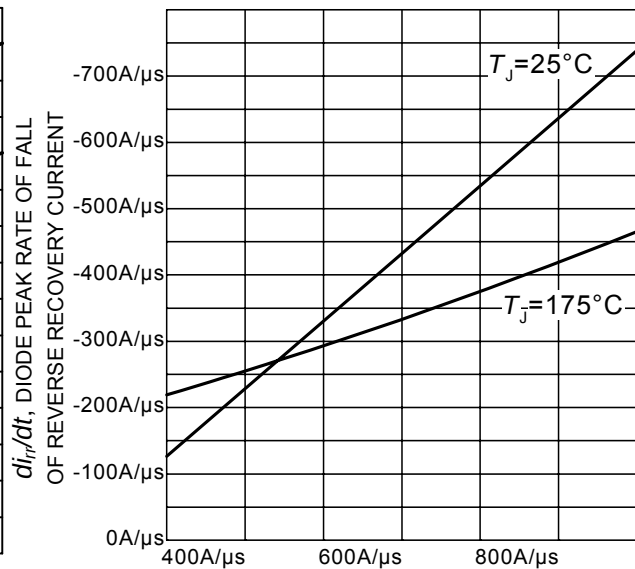
Figure 26. Typical diode peak rate of fall of reverse recovery current as a function of diode current slope ( V_R = 400V , I_F = 10A , Dynamic test circuit in Figure E)
