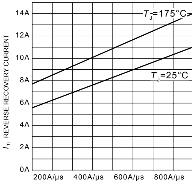
Figure 25. Typical reverse recovery current as a function of diode current slope ( V_R = 400V , I_F = 10A , Dynamic test circuit in Figure E)
