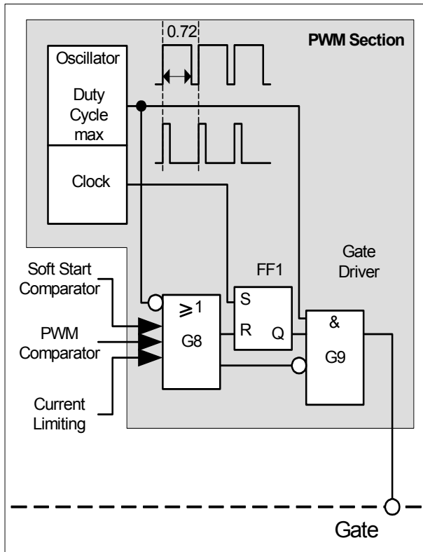
Figure 7 PWM Section
