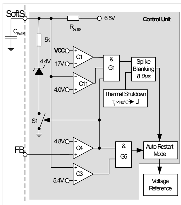
Figure 18 Auto Restart Mode
