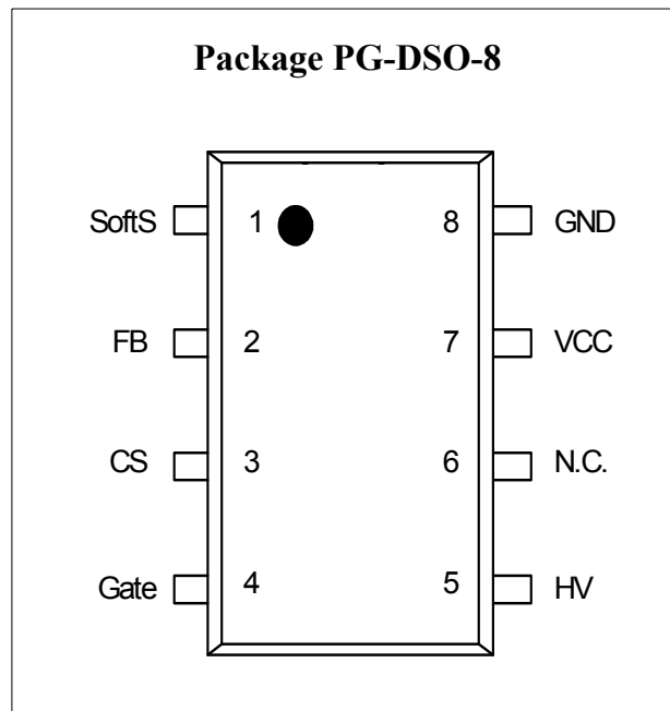
Figure 2 Pin Configuration PG-DSO-8(top view)
