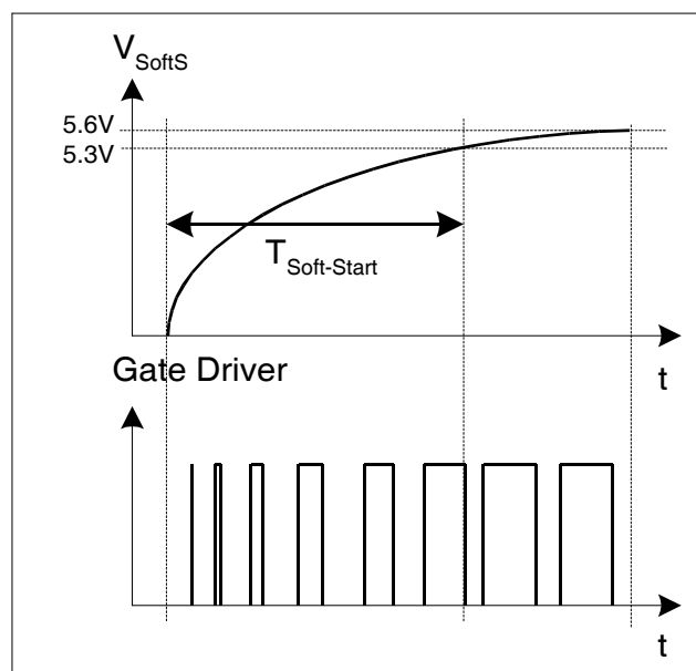
Figure 12 Soft-Start Phase
