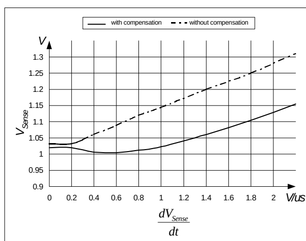
Figure 19 Overcurrent Shutdown
