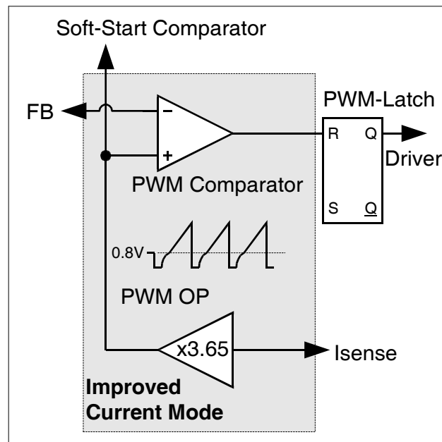
Figure 7 Current Mode
