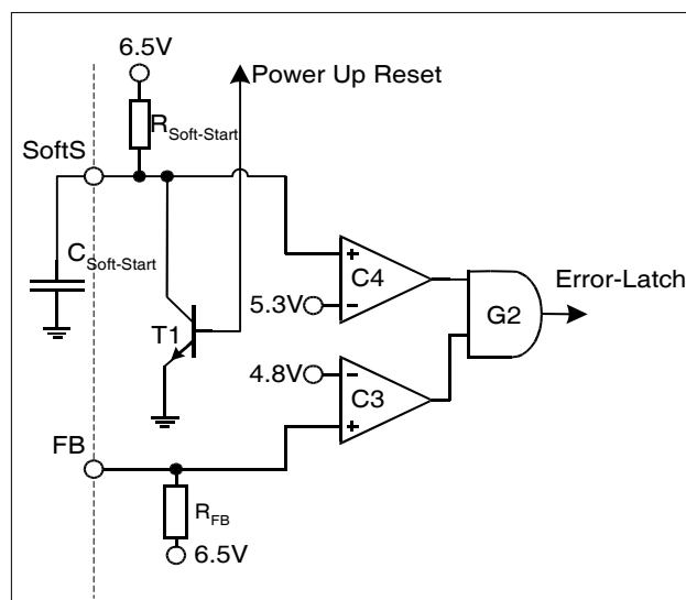
Figure 22 FB-Detection
