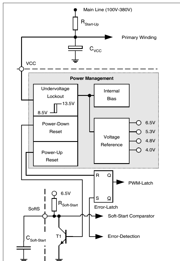
Figure 6 Power Management
