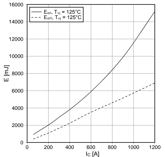
Schaltverluste IGBT-Wechselr. (typisch) switching losses IGBT-inverter (typical) E_{on} = f(I_C) , E_{off} = f(I_C) V_{GE} = \pm 15\text{ V} , R_{Gon} = 4.3\ \Omega , R_{Goff} = 30\ \Omega , V_{CE} = 3600\text{ V} , C_{GE} = 68\text{ nF}
