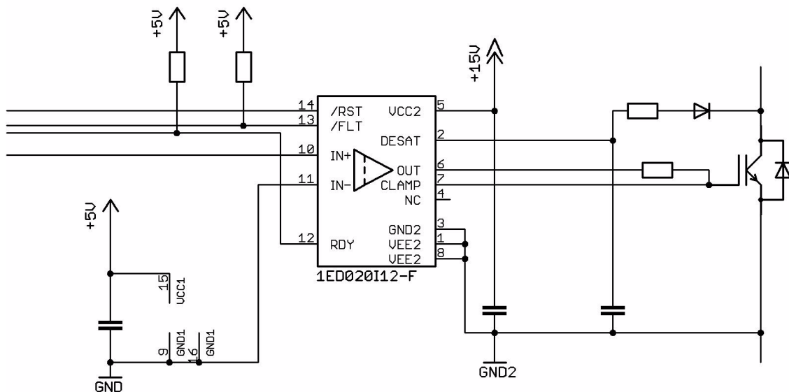
Figure 3: Application example
