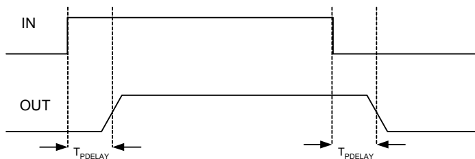
Figure 5: Propagation Delay
