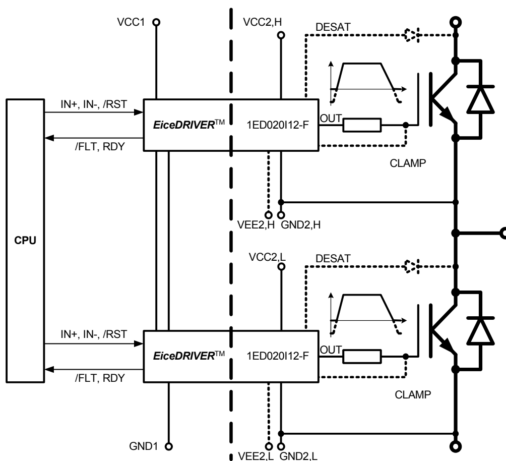
Figure 1: Typical Application
