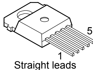
TO-218AB/5
