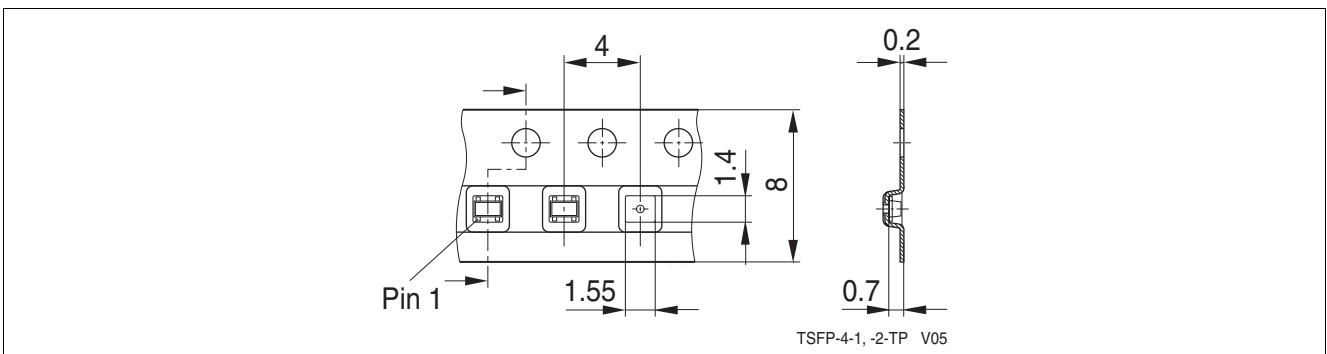
Figure 9-4 Tape dimensions
