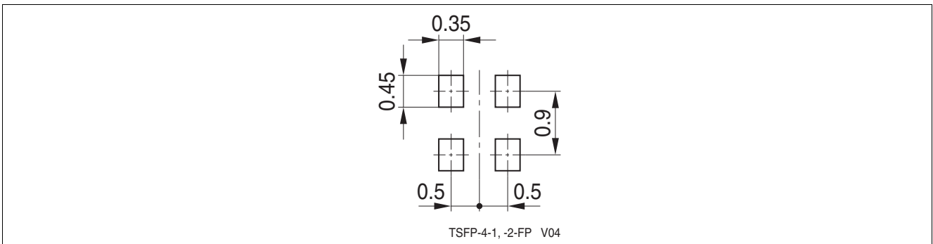
Figure 9-2 Package Footprint
