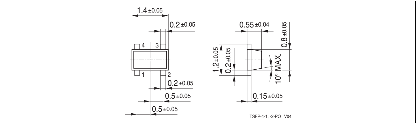
Figure 9-1 Package Outline
