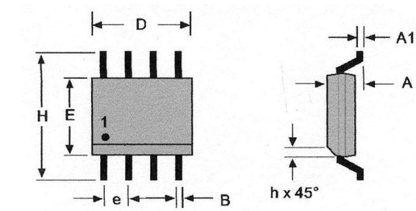
PACKAGE DRAWING HMC1501/HMC1512 (8-PIN SOIC, dimensions in millimeters)
