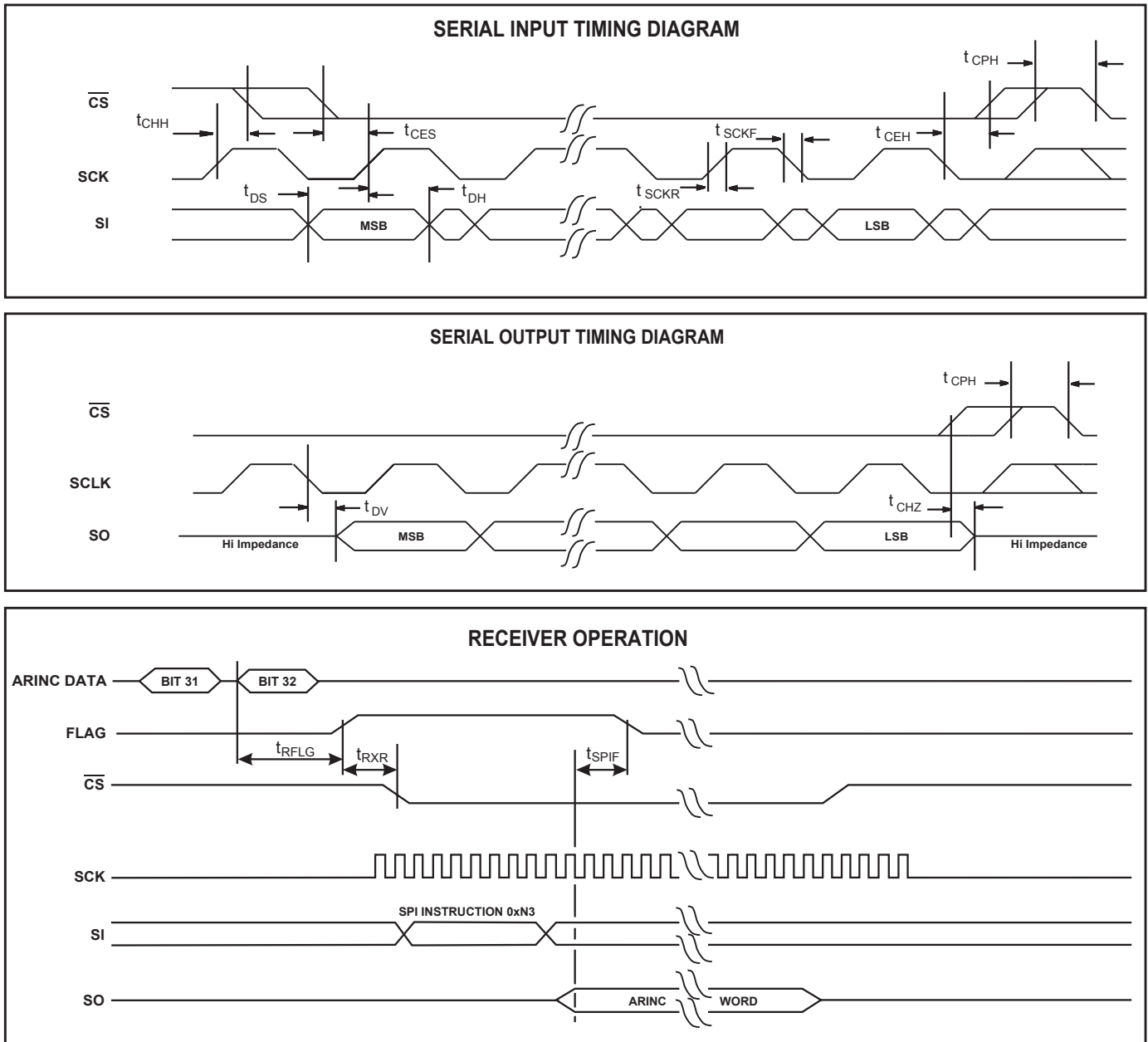
Figure 5. Timing Diagrams
